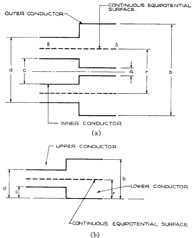
Fig. 8. Location of continuous equipotential surface through double discontinuity. (a) Double step in coaxial line. (b) Double step in parallel plate line.
