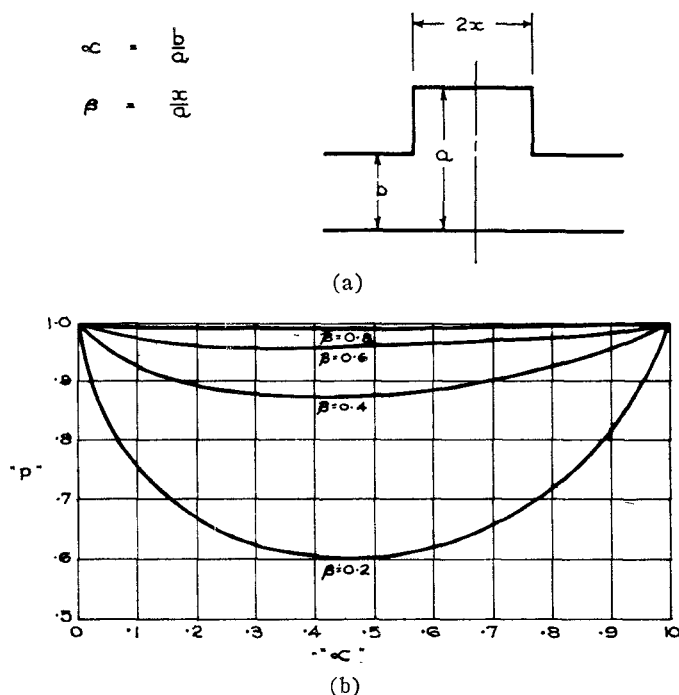
Fig. 9. Proximity factor for double step in parallel plate line. (a) Notation. (b) Proximity-factor curves.
