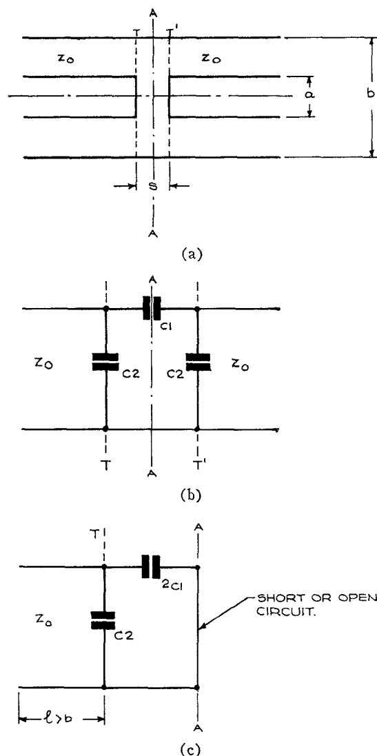
Fig. 10. Series gap in coaxial line and equivalent circuit. (a) Series gap in coaxial line. (b) Equivalent circuit of gap. (c) Circuit for analysis.
